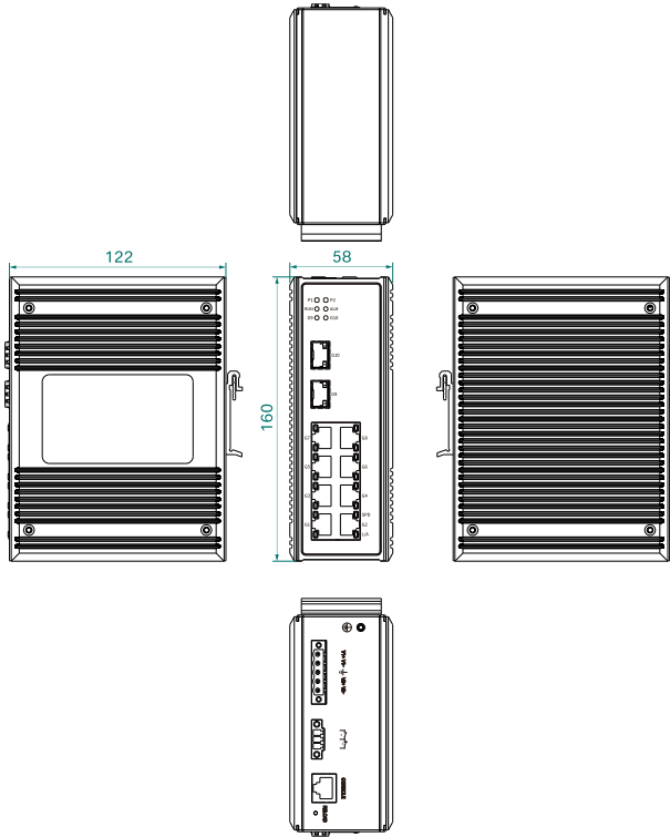
MISCOM7210G-2GF-8GT
