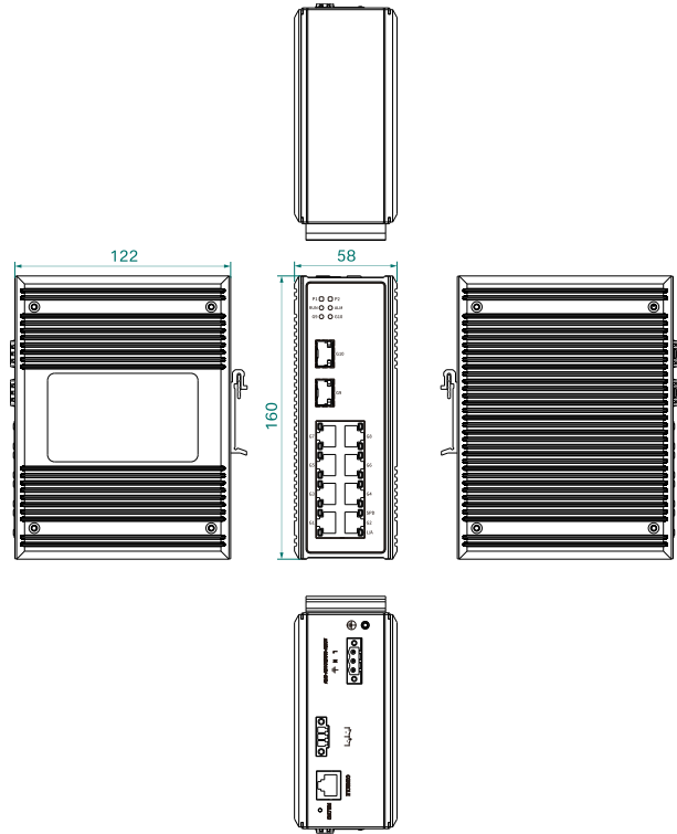
MISCOM7210G-2GF-8GT-AD220
